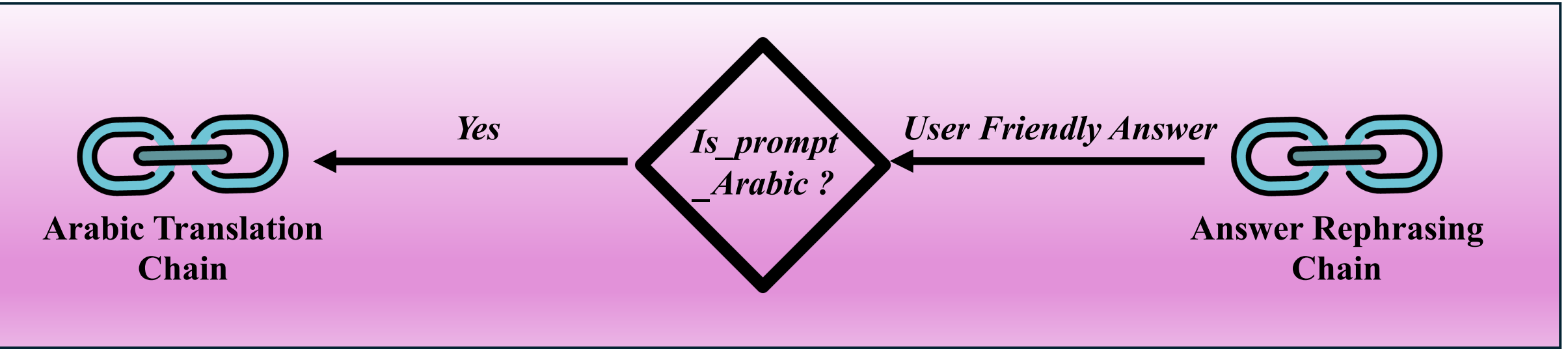
Final Answer
