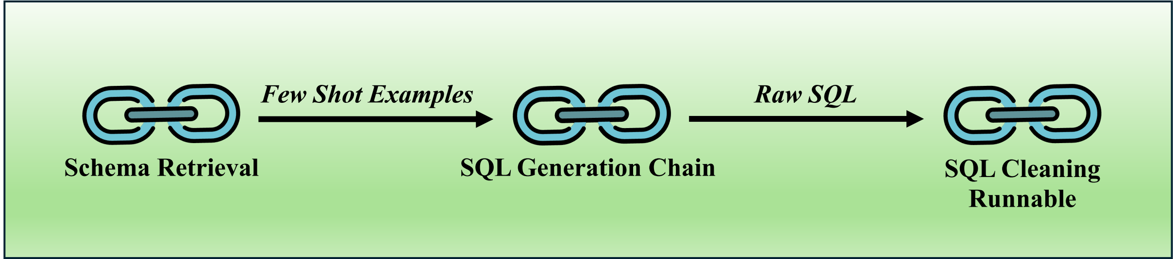
Query Generation
