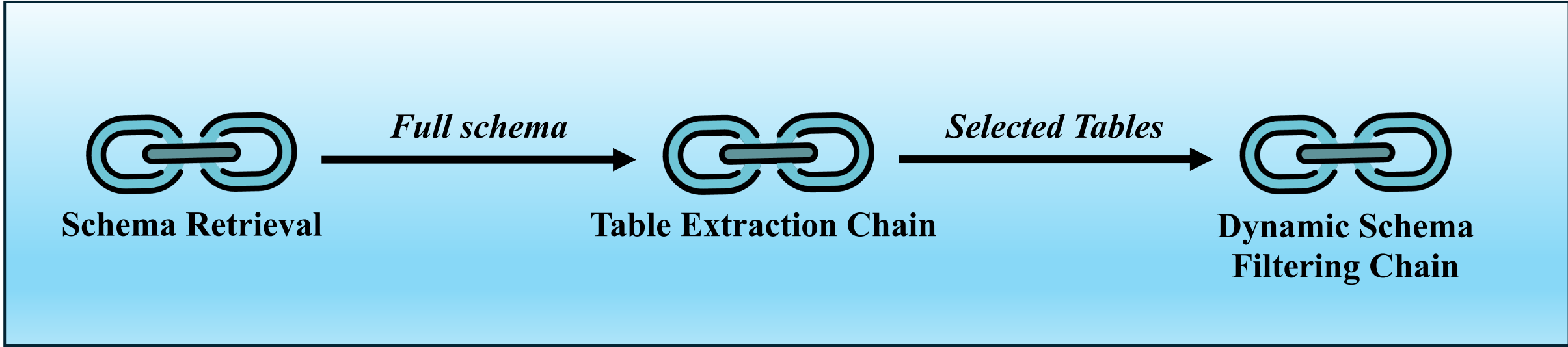
Schema Processing
