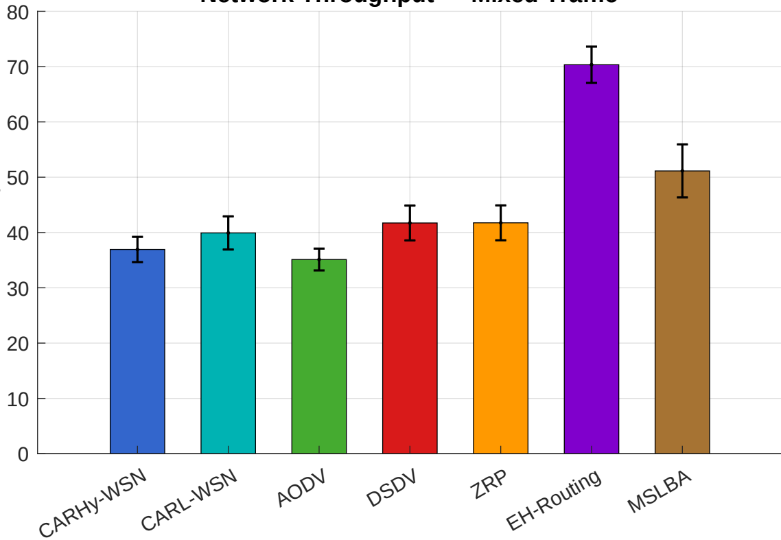
Network Throughput — Mixed Traffic
