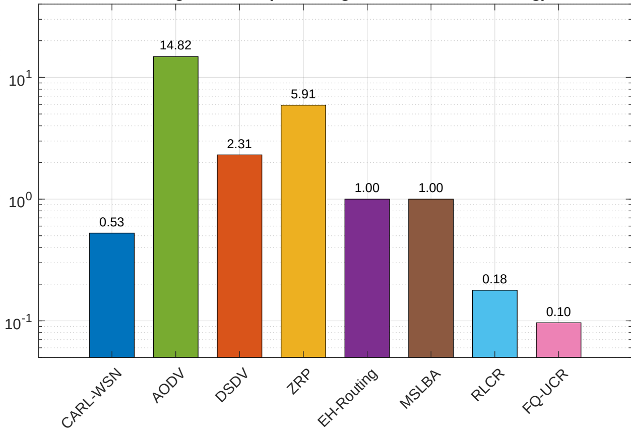
Routing Overhead (clustering under TDMA accounting)
