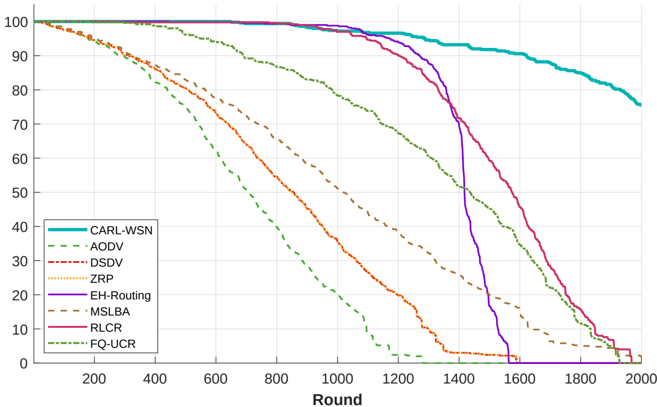
Network Lifetime — Alive Nodes Over Time
