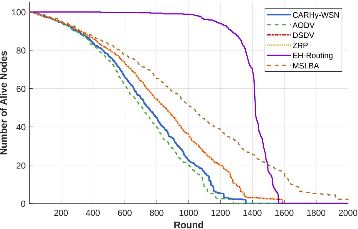
Network Lifetime — Alive Nodes Over Time
