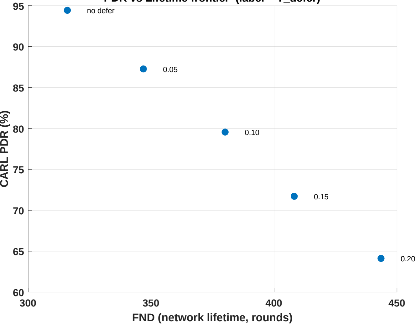
PDR vs Lifetime frontier (label = T_defer)
