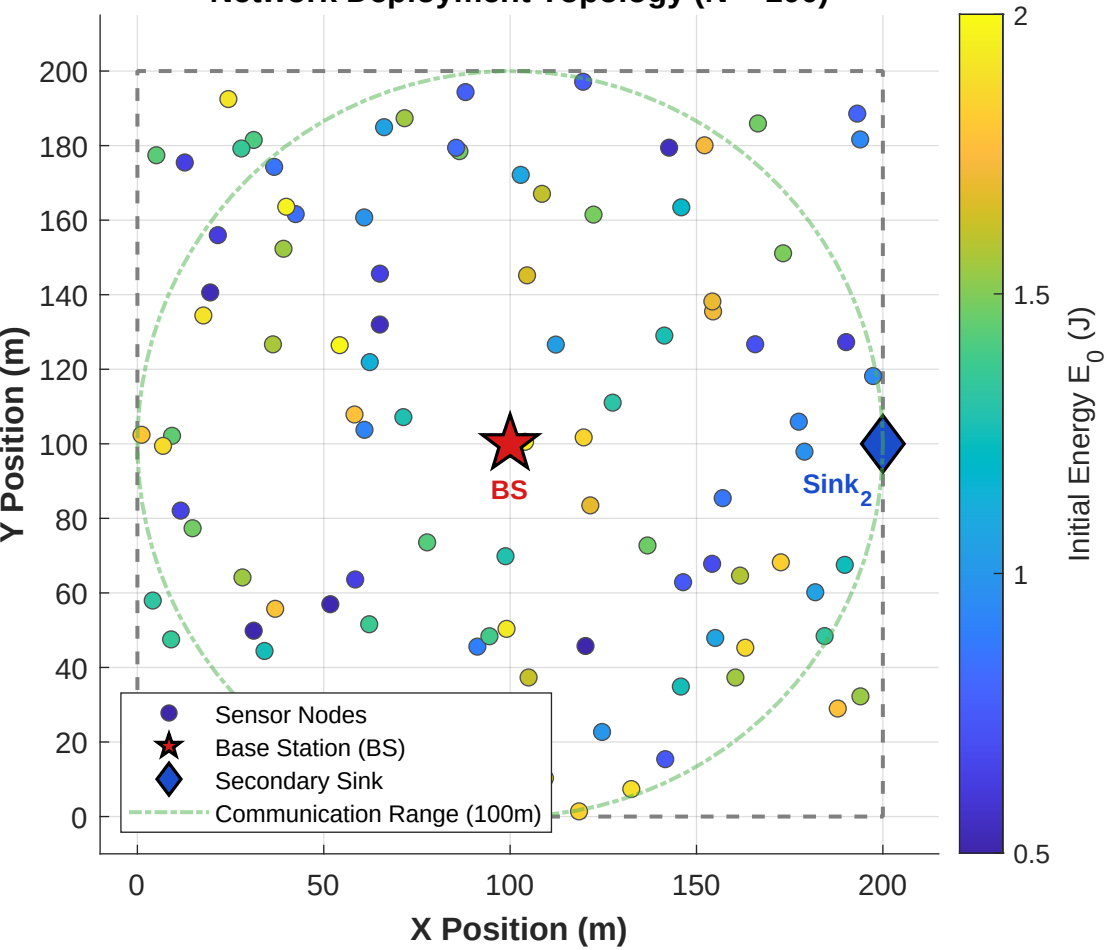
Network Deployment Topology (N = 100)
