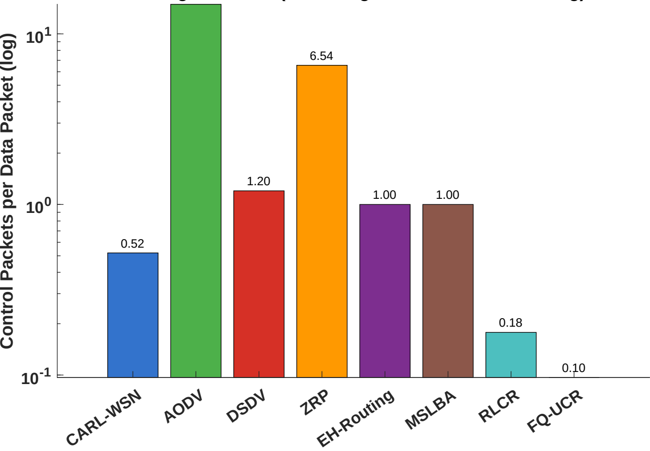
Routing Overhead (clustering under TDMA accounting)
