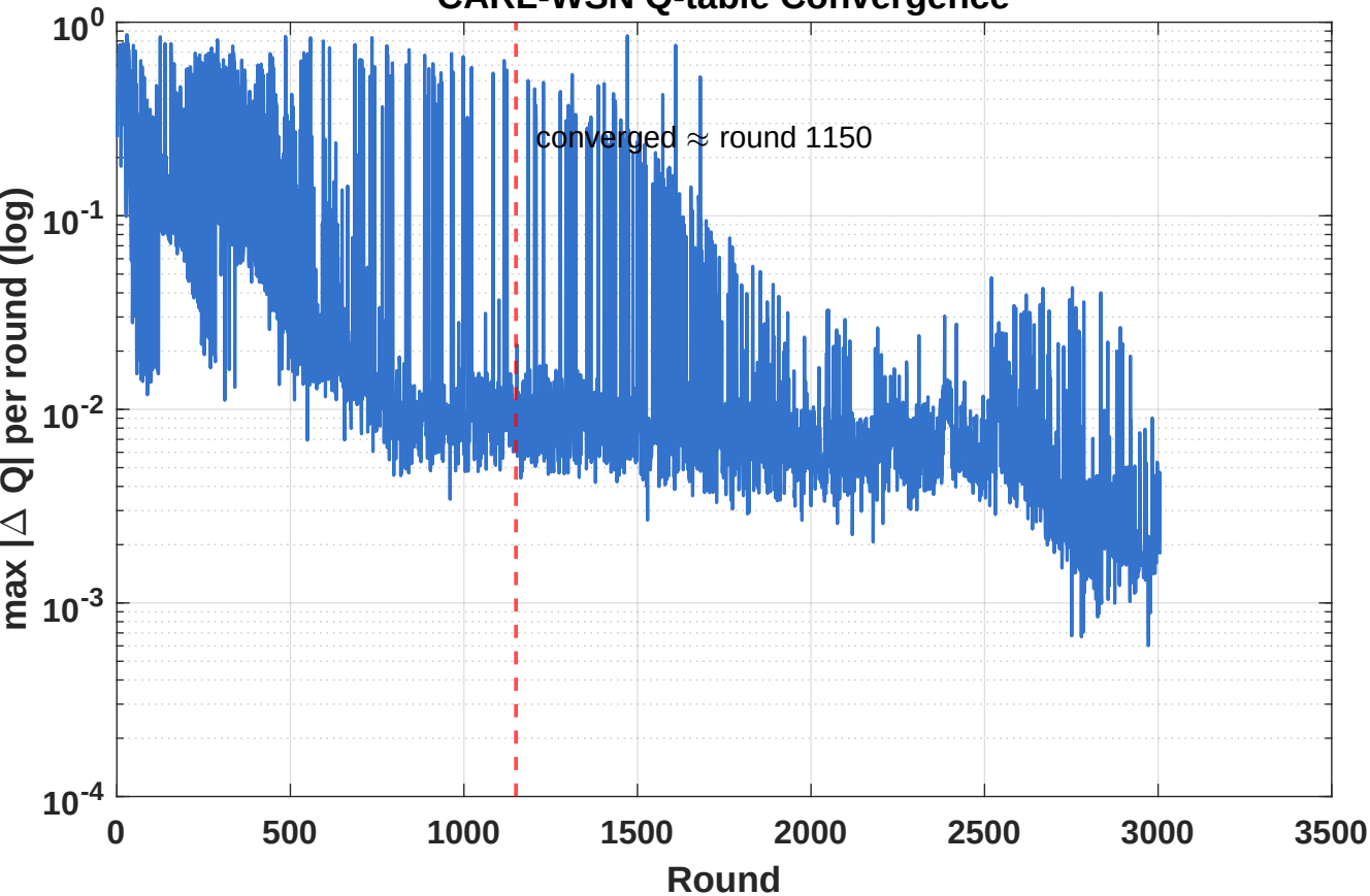
CARL-WSN Q-table Convergence
