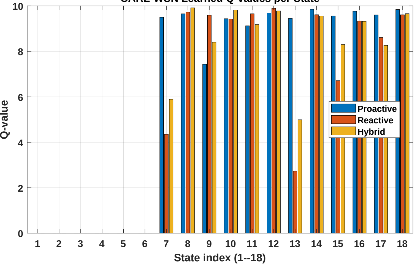
CARL-WSN Learned Q-values per State
