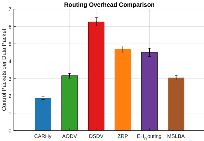
Fig. 2. Routing overhead (control packets per data packet). CARHy-WSN achieves the lowest overhead, with 70.2% reduction vs. DSDV.
