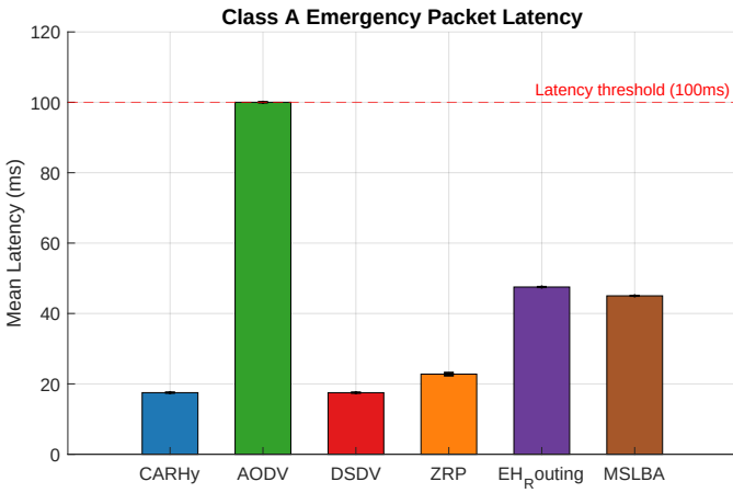
Fig. 1. Mean Class A emergency packet latency. CARHy-WSN achieves 82.5% reduction compared to AODV. Error bars show standard deviation across five independent runs.
