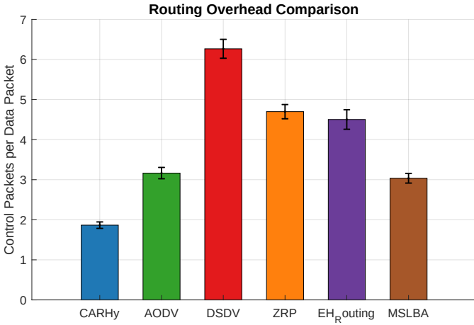
Fig. 2. Routing overhead (control packets per data packet). CARHy-WSN achieves the lowest overhead, with 70.2% reduction vs. DSDV.
