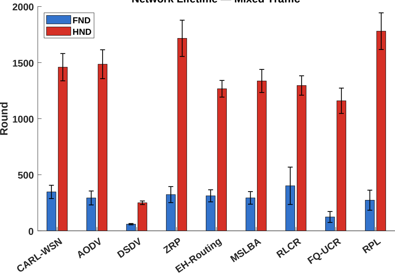
Network Lifetime — Mixed Traffic
