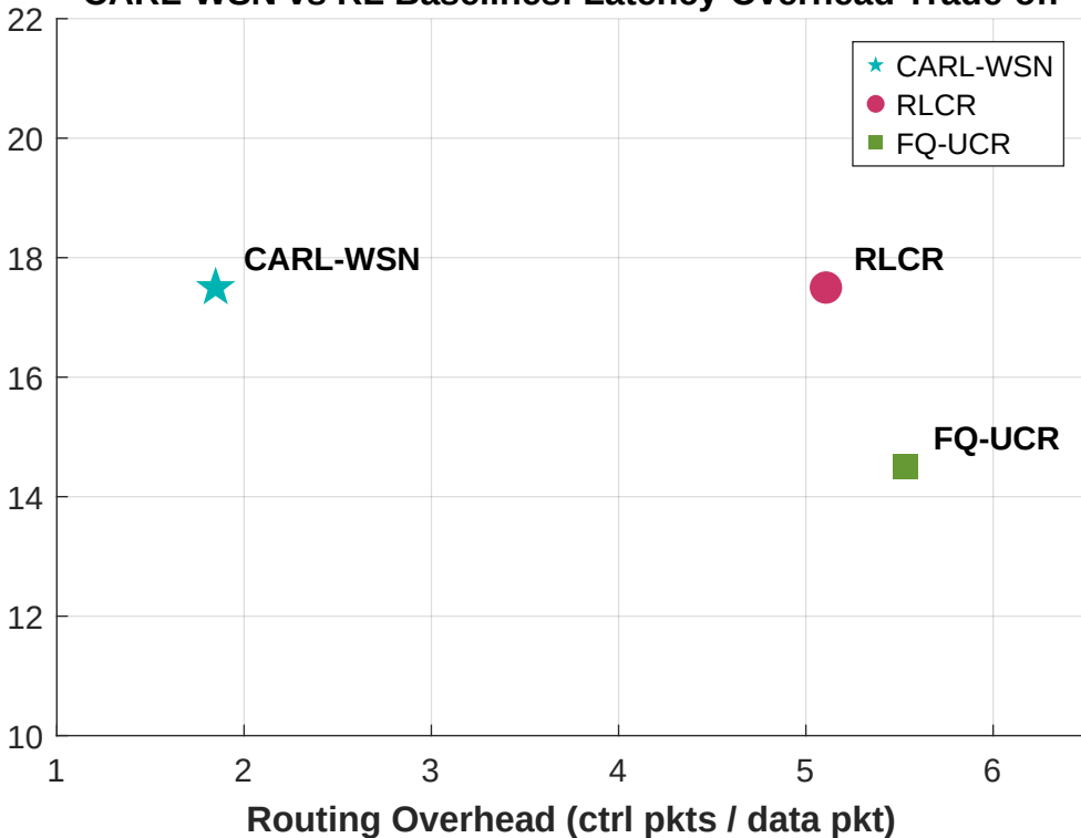
CARL-WSN vs RL Baselines: Latency-Overhead Trade-off
