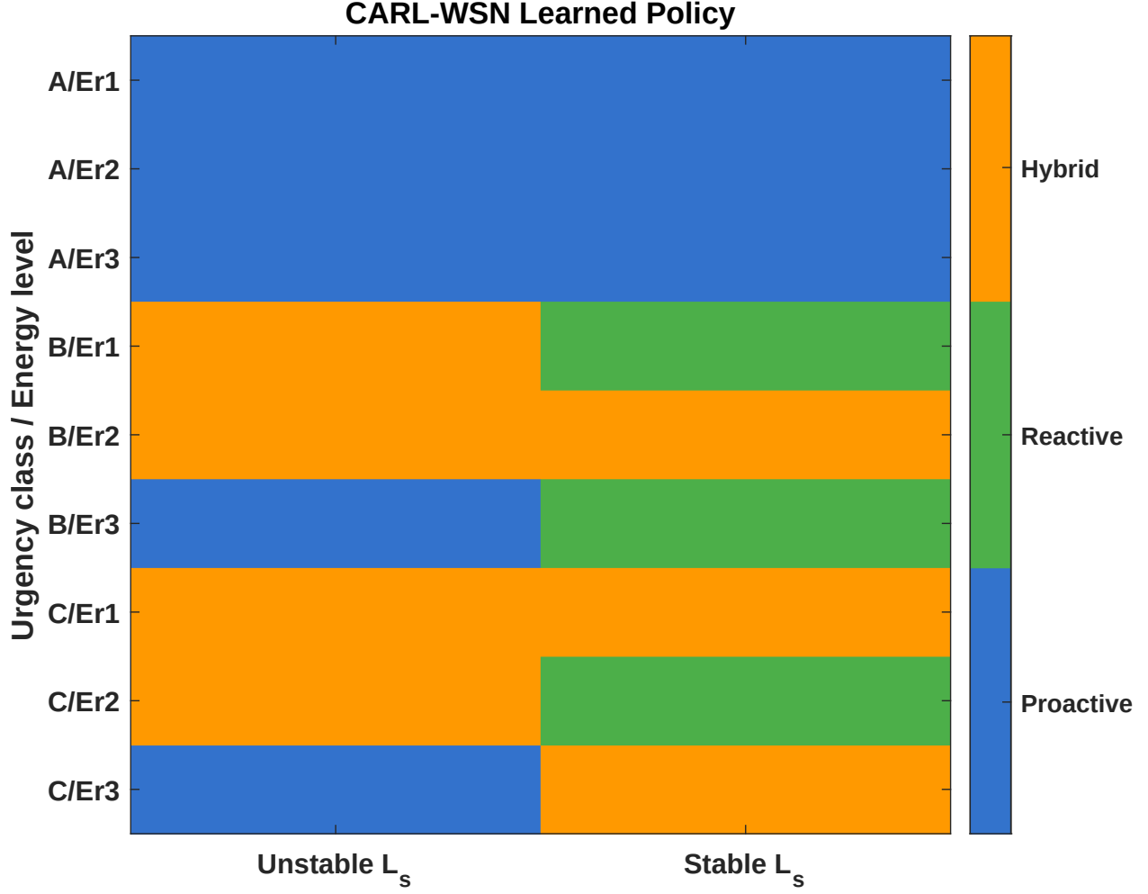
Figure 8: CARL-WSN routing policy across all 18 context states. Left: unstable link ( L_s < 0.7 ). Right: stable link ( L_s \geq 0.7 ). Blue = proactive, green = reactive, orange = hybrid. States 1–6 (Class A) are fixed by the hardcoded safety constraint, not learned; the agent learns class-dependent and context-dependent routing strategies for the remaining 12 states (Class B/C).
