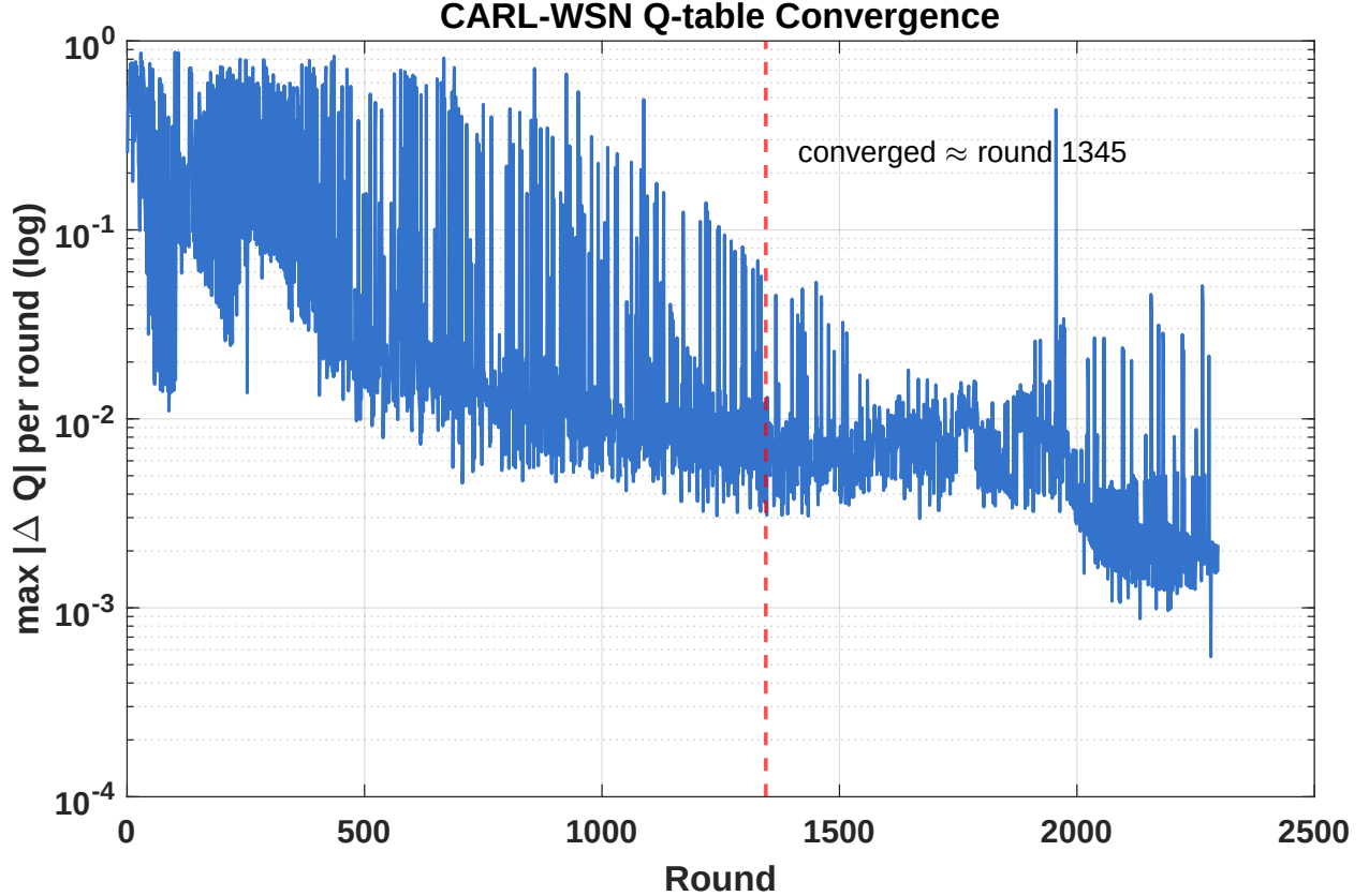
Figure 7: CARL-WSN Q-table convergence: maximum Q-value update per round (log scale). The agent converges to a stable policy within approximately 1345 rounds.
