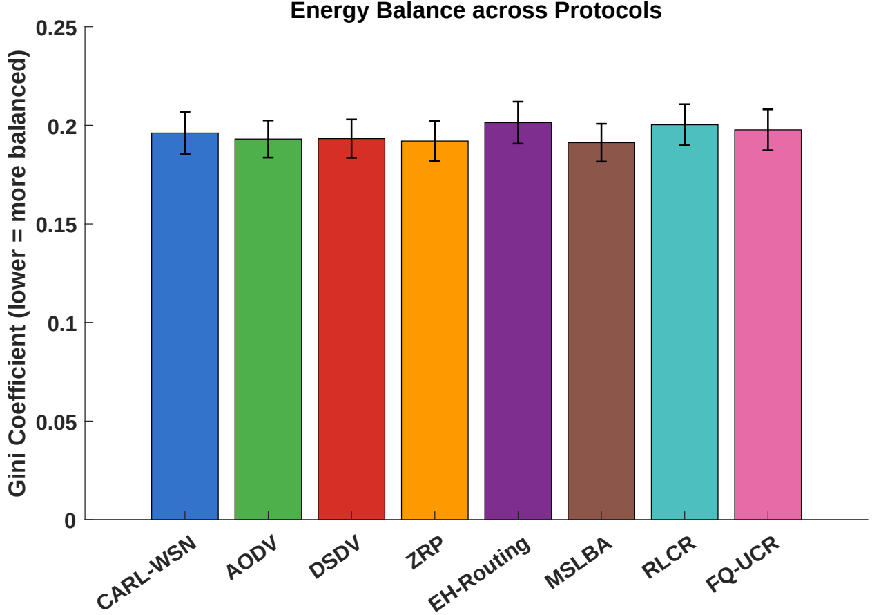
Figure 5: Gini coefficient of per-node energy consumption (lower is more balanced). Values are tightly clustered (0.191–0.201); the omnibus ANOVA is marginally significant ( p = 0.043 ), driven solely by the EH-Routing versus MSLBA pair, and no comparison involving CARL-WSN (0.196) is significant.
