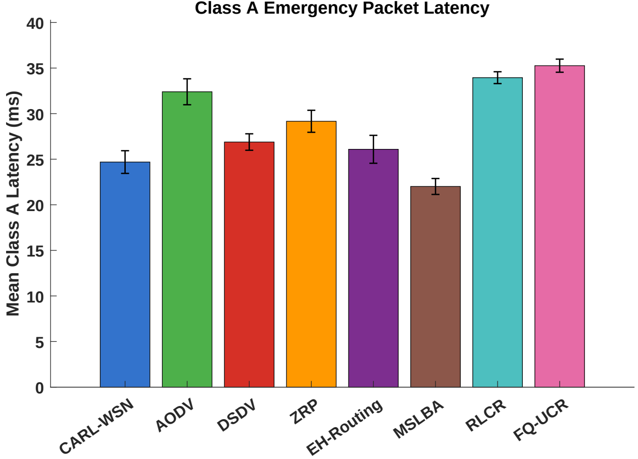
Figure 2: Mean Class A emergency packet latency under mixed traffic. CARL-WSN achieves a 23.8% reduction versus AODV and remains among the lowest-latency protocols, all within the 100 ms emergency deadline. Error bars show standard deviation across 20 independent seeds.
