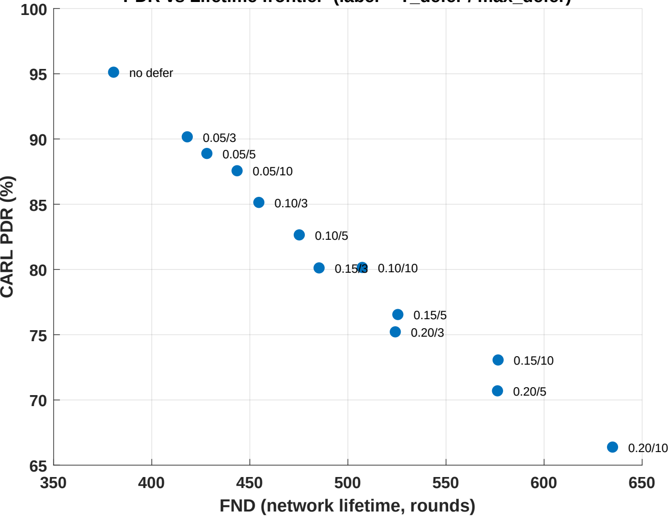
PDR vs Lifetime frontier (label = T\_defer / \max\_defer )
