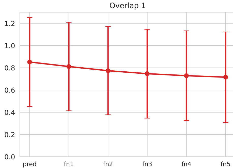
Topological Distance to Ground Truth (predicted → finetune epochs)
