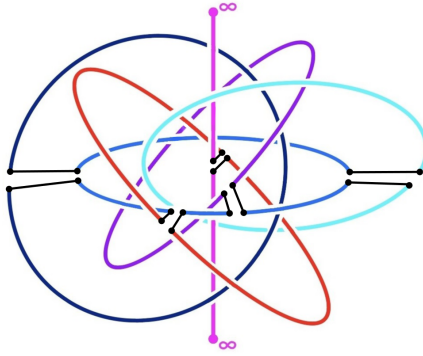
FIGURE 3. Connecting the disjoint circles comprising \Pi^{-1}(O) to form a path-connected figure \Gamma_O in accordance with the tree \mathcal{T}_O as in Figure 2. This is the image of a (\frac{5\pi+\delta}{12\pi}, \frac{1}{12\pi}) -approximate 7-design curve, with \delta as in Proposition 3.1.
