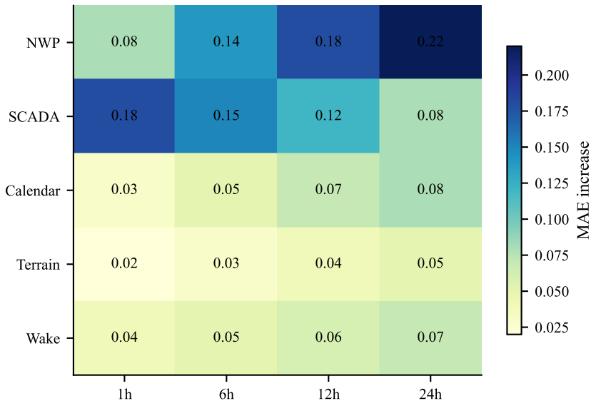
Ablation links feature groups to horizon
