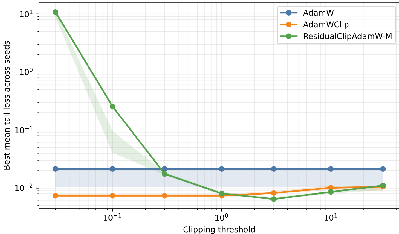
Best loss after learning-rate and momentum selection (lines: mean; bands: seed IQR)
