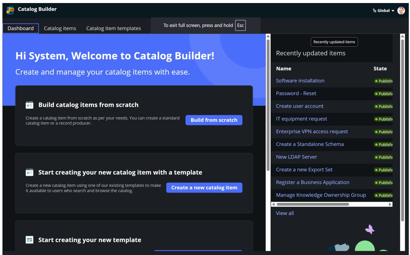
Figure 4.2: Catalog Builder
