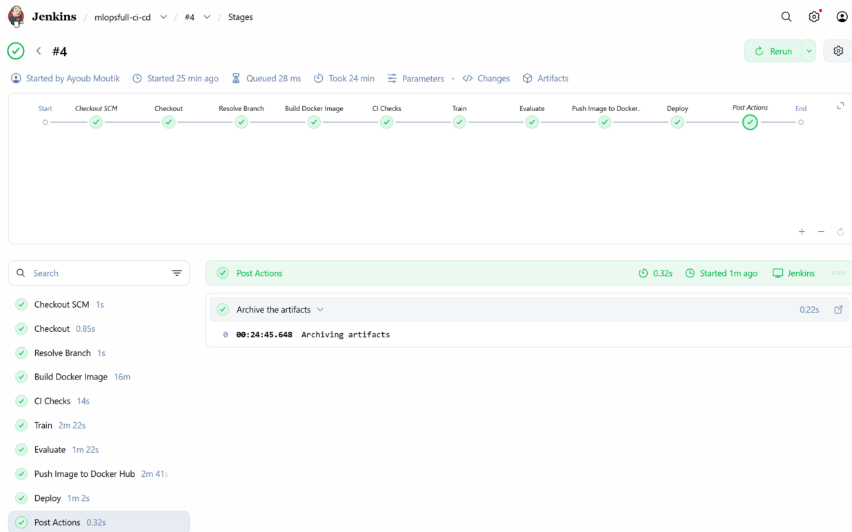
Figure 6: Jenkins build evidence showing all CI/CD stages completed successfully.
