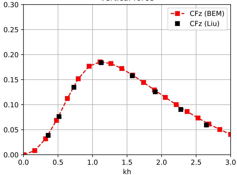
Vertical force
