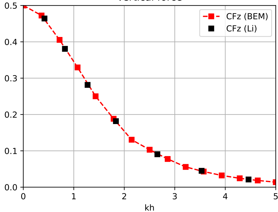
Vertical force
