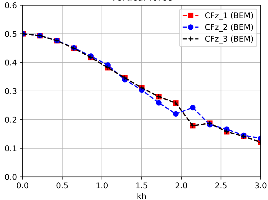
Vertical force
