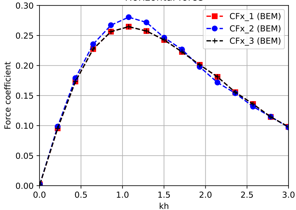
Horizontal force
