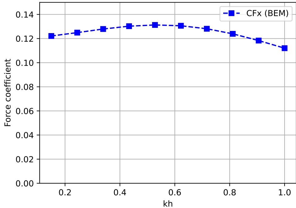
Horizontal force
