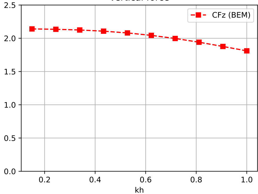
Vertical force
