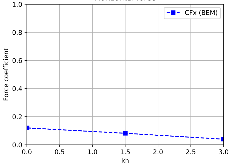
Horizontal force
