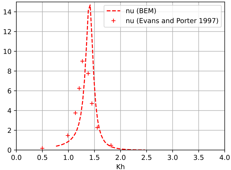
Radiation conductance
