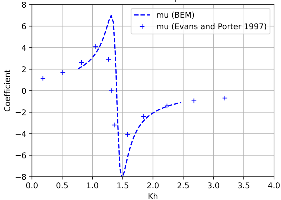
Radiation susceptance
