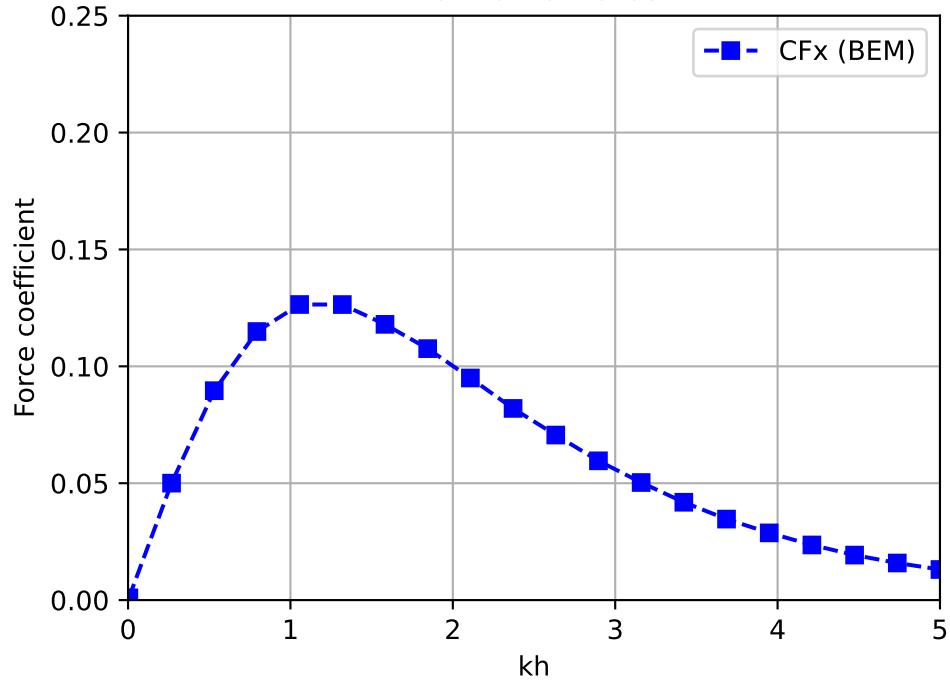
Horizontal force
