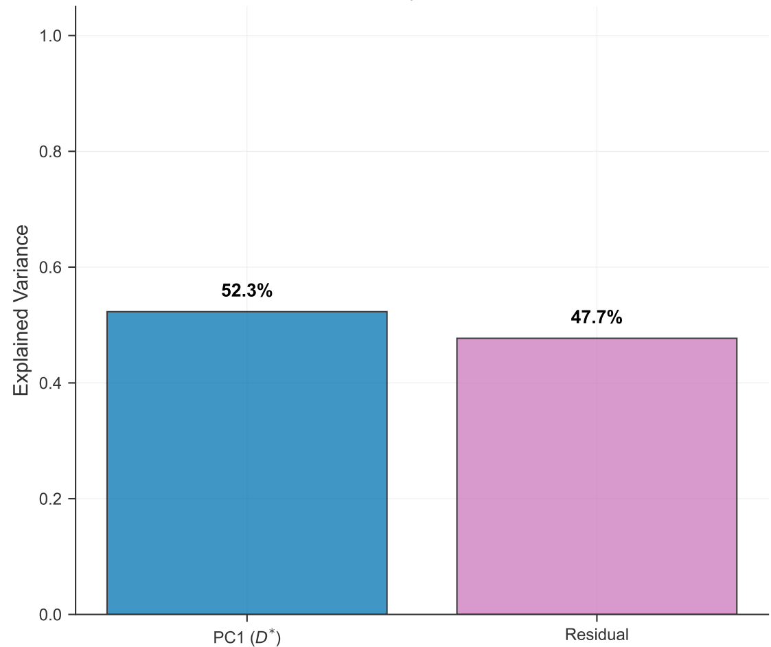
Variance Explained by Principal Components
