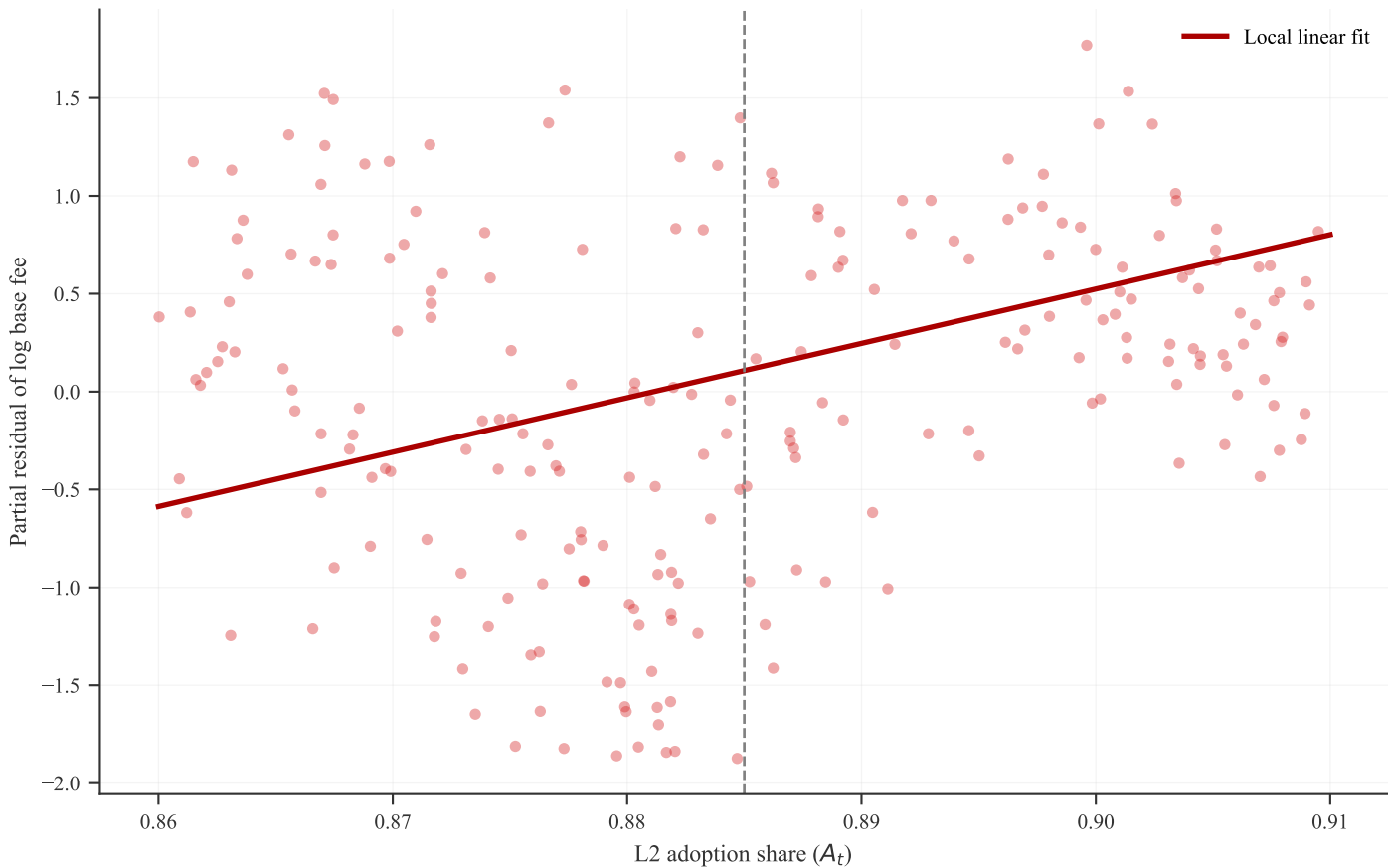
Local Post-Dencun Fit within [0.86, 0.91]
