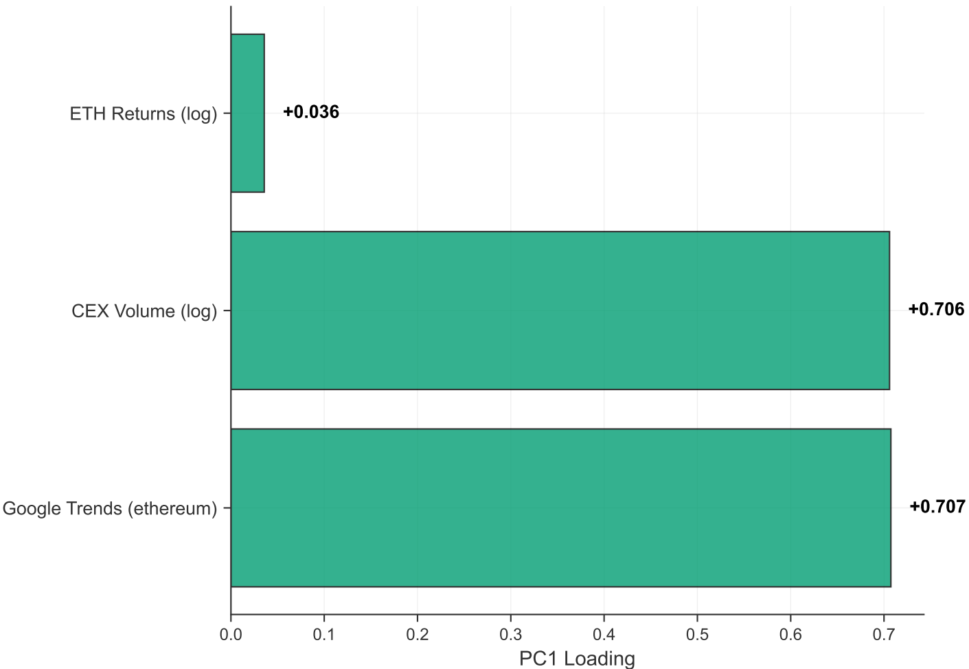
PC1 Loadings ( D^* -lite)
