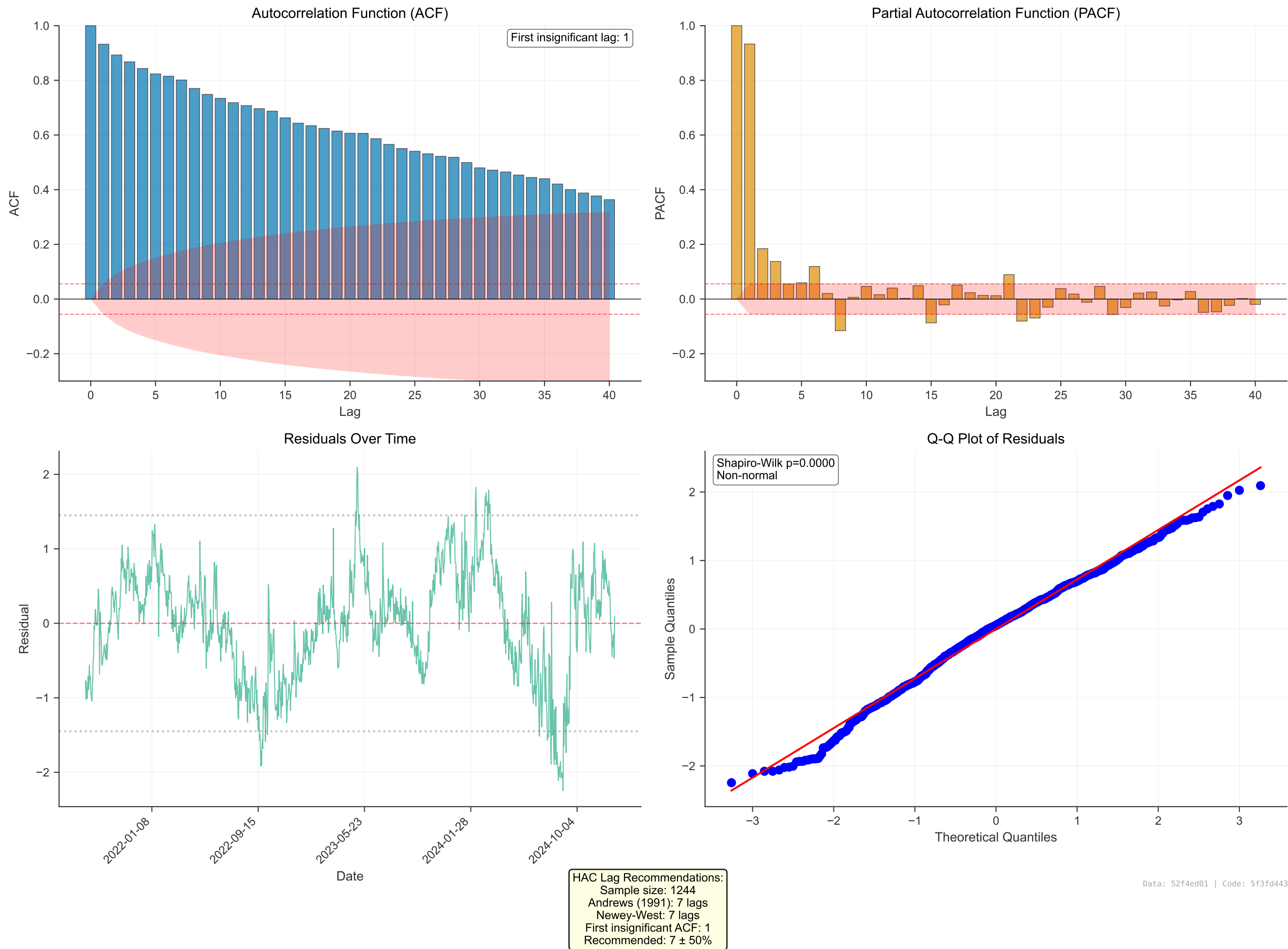
Figure 7: Residual Diagnostics for HAC Lag Selection
