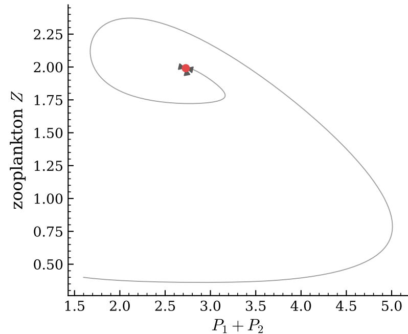
(a) below the Hopf, \iota_0 = 0.5
