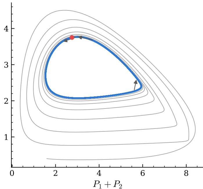
(b) above the Hopf, \iota_0 = 0.85
