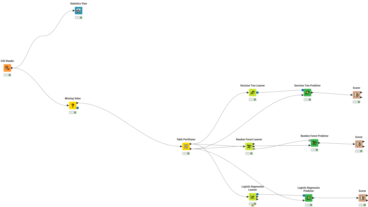
Figure 4. I extracted this completed workflow preview from my exported DemoEarlyWarningTool.knwf file. It shows my CSV Reader and preprocessing flow, Table Partitioner, and the Decision Tree, Random Forest, and Logistic Regression learner-predictor-scorer branches.
