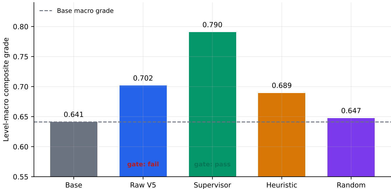
Average grade and release-gate outcome are different signals
