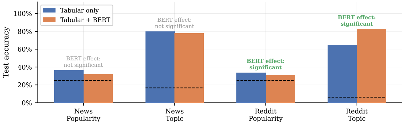
Tabular-only vs. tabular+BERT accuracy across the 2 \times 2 study grid (dashed line = chance level; significance = paired bootstrap test, \alpha = 0.05 , n = 2000 resamples)
