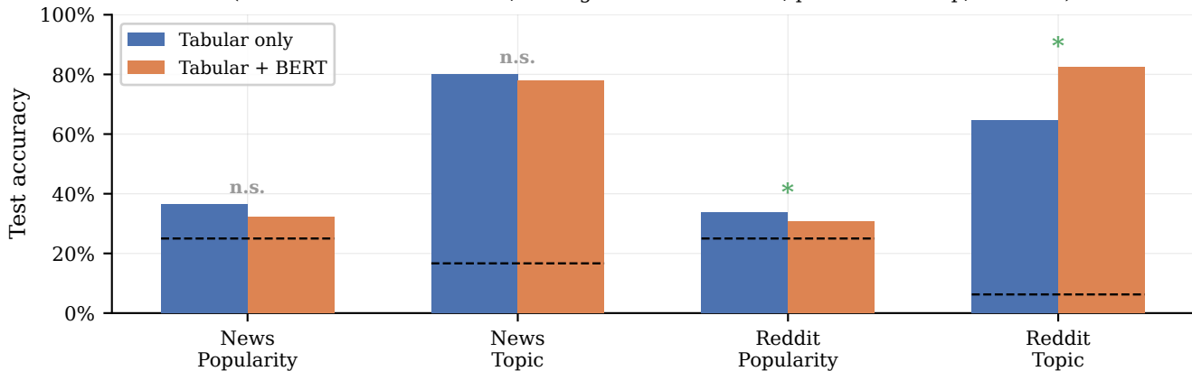
Tabular-only vs. tabular+BERT accuracy across the 2 \times 2 study grid (dashed line = chance level; * = significant at \alpha = 0.05 , paired bootstrap, n = 2000 )
