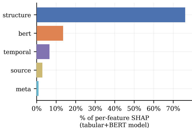
Popularity
