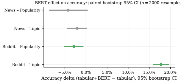
Fig. 3. Paired-bootstrap 95% confidence intervals on the accuracy delta. Only the two Reddit cells exclude zero.
