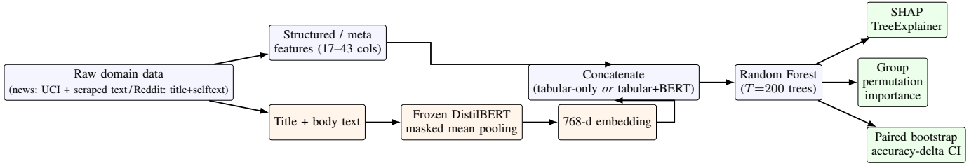
Fig. 1. Shared pipeline. Both feature configurations (tabular-only, tabular+BERT) and all four task/domain cells run this exact pipeline; only the input feature set, the label, and the classifier’s random-forest hyperparameters (depth cap, Reddit only, §IV-D) differ.
