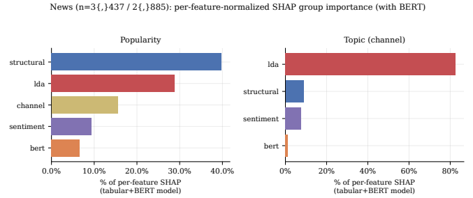
Fig. 4. News domain: per-feature-normalized SHAP group importance, tabular+BERT model. Structural features dominate popularity; LDA dominates topic. BERT is not the top group in either task.
