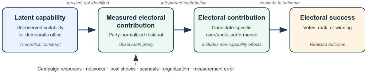
Figure 1: Measurement model. The residual is an observable proxy for latent capability and an election-specific index of measured electoral contribution; it is neither latent capability itself nor realized electoral success.
