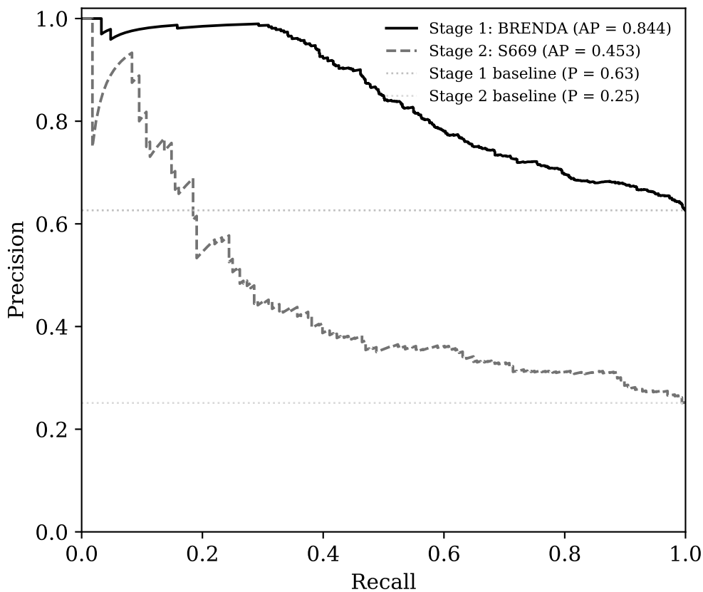
Precision-recall curves
