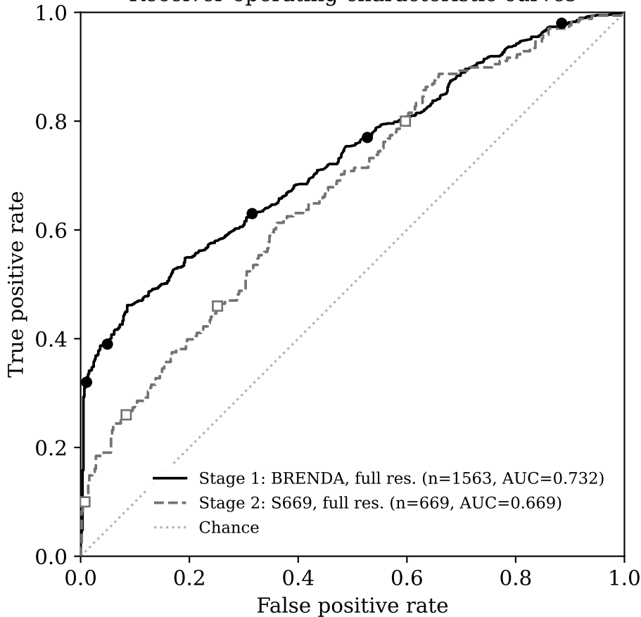
Receiver-operating-characteristic curves
