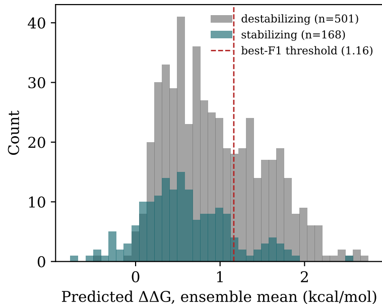
Predicted-score distribution by true label
