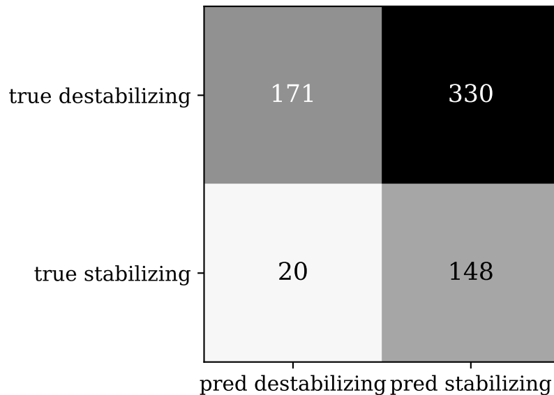
Confusion matrix @ 1.16 kcal/mol (best F1 = 0.46)
