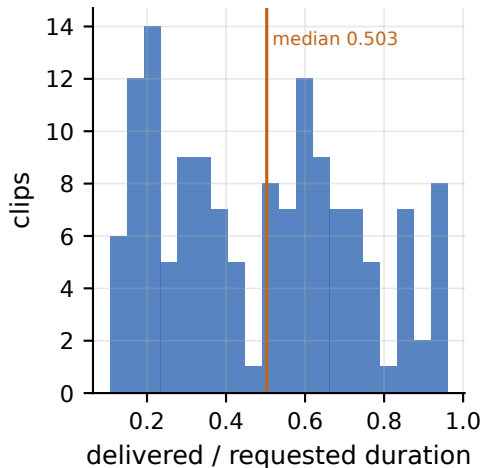
duration retention (n=141)
