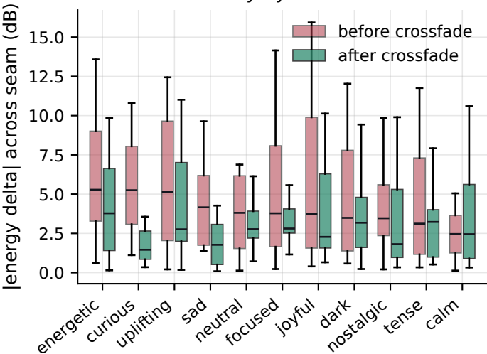
seam discontinuity by mood
