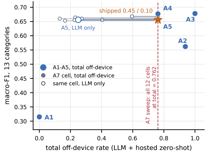
Fig. 4. Macro-F1 against total off-device rate for A1–A5 and a twelve-cell threshold sweep. Filled points (total off-device) stack at .762 regardless of threshold; hollow points (LLM-only exposure) spread .13–.60.
