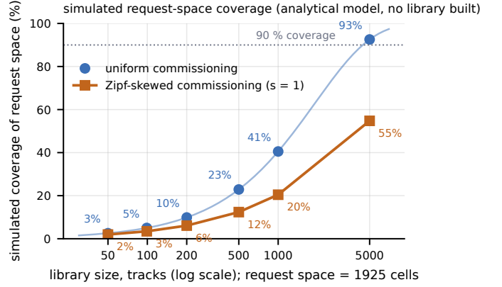
Fig. 5. Simulated coverage against library size, uniform and skewed commissioning. Analytical, not empirical.
