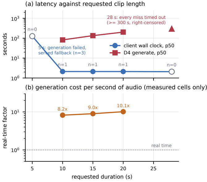
Fig. 3. Generation latency against requested duration (a) and real-time factor (b). Filled squares are the three completed generations; open markers are cells no request reached (28 s: every miss timed out, a lower bound at 300 s).
