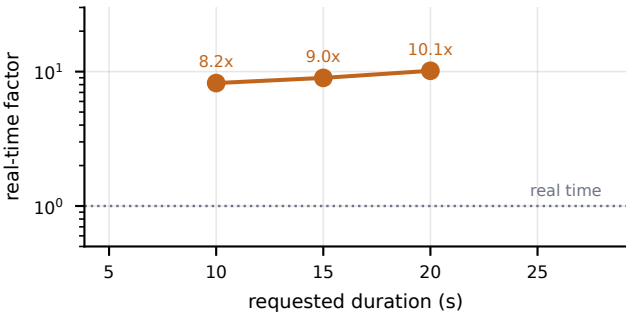
(b) generation cost per second of audio (measured cells only)
