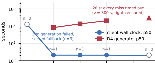
(b) generation cost per second of audio (measured cells only)
