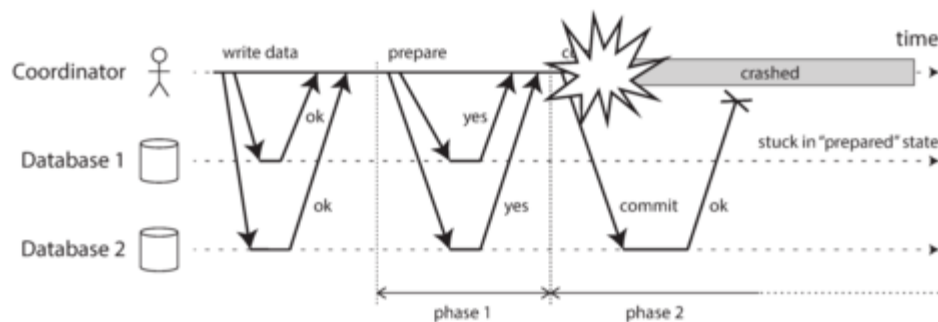
Figure 9-10. The coordinator crashes after participants vote “yes.” Database 1 does not know whether to commit or abort.
