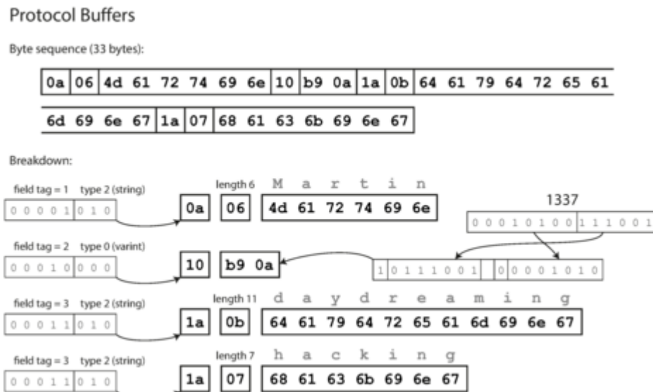
Figure 4-4. Example record encoded using Protocol Buffers.
