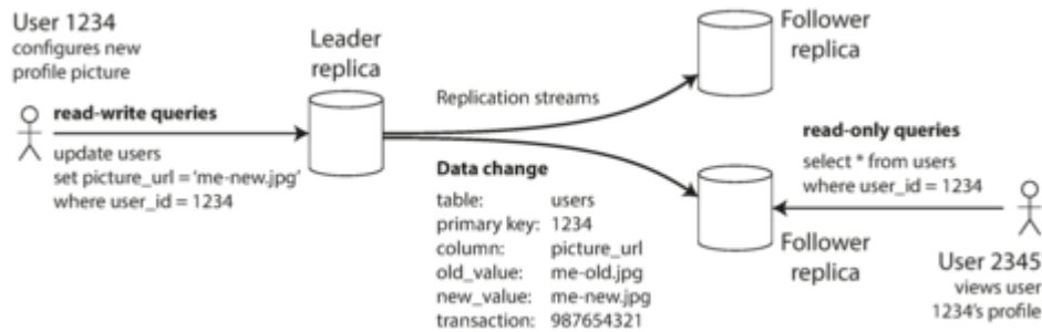
Figure 5-1. Leader-based (master–slave) replication.
