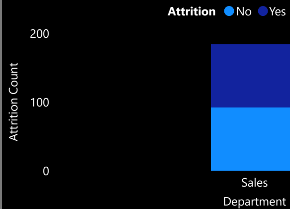
ATTRITION COUNT BY DEPARTMENT AND ATTRITION
