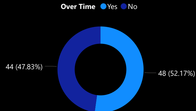
ATTRITION COUNT BY OVERTIME
