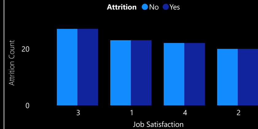
ATTRITION COUNT BY JOB SATISFACTION AND ATTRITION
