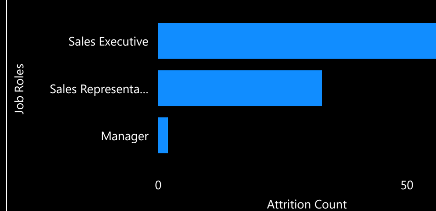
ATTRITION COUNT BY JOB ROLE
