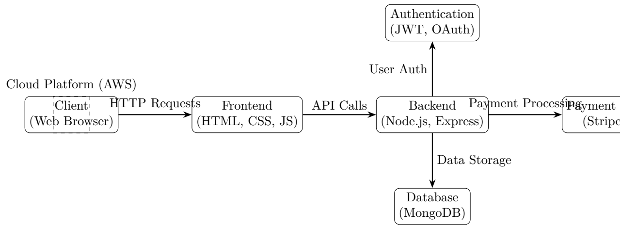
Figure 1: Architectural Diagram of One-Day Subscription Service
