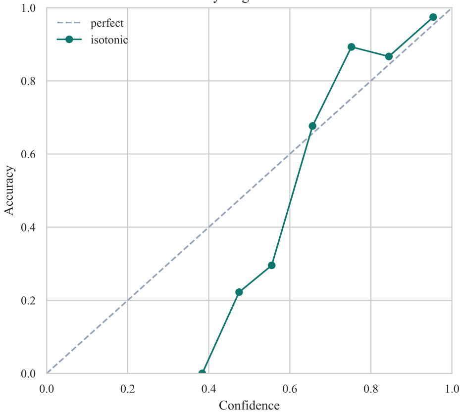
Reliability diagram — isotonic
