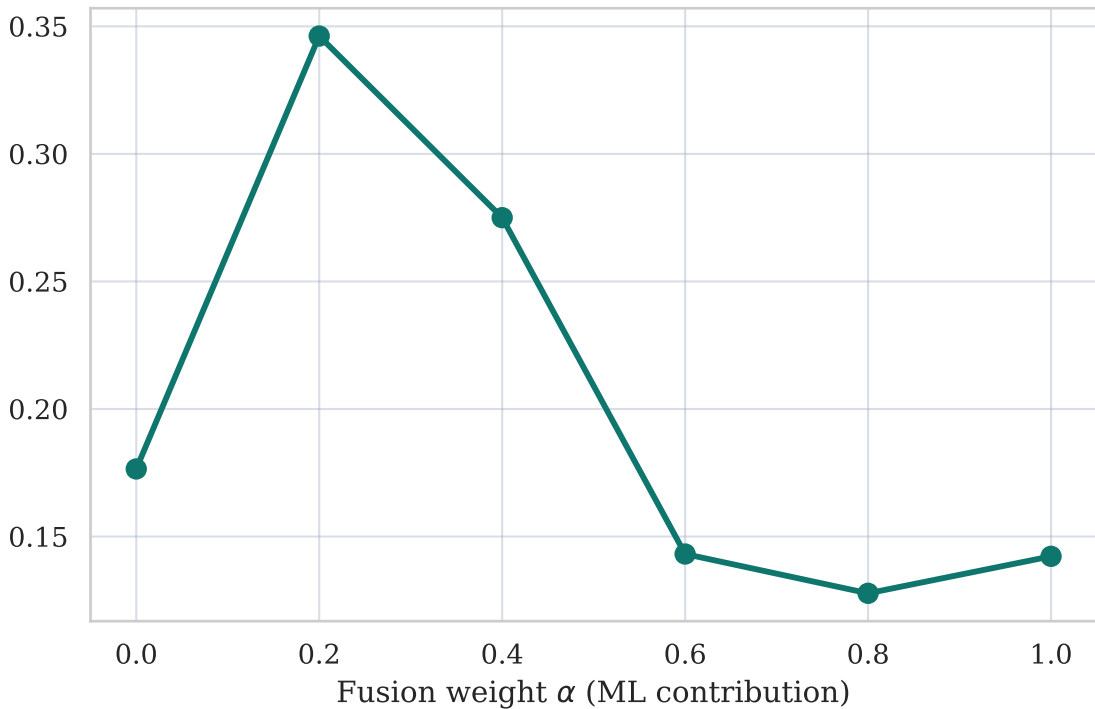
Expected Calibration Error
